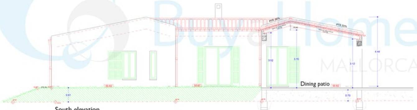
South elevation
