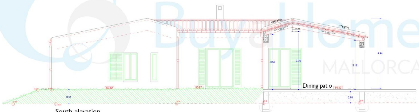
South elevation
